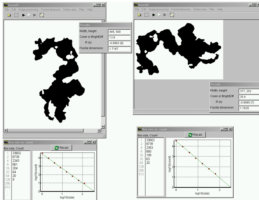
Fig. 1 – Fractal Dimension Calculator
